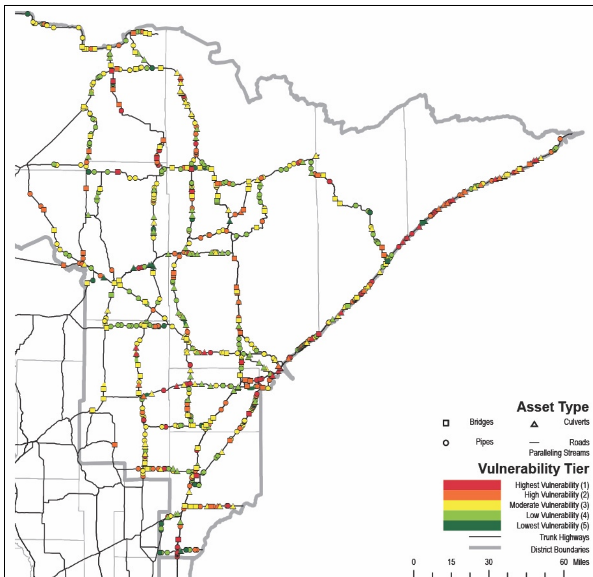
Asset vulnerability to flash flood events in MnDOT District 1. Source: MnDOT
