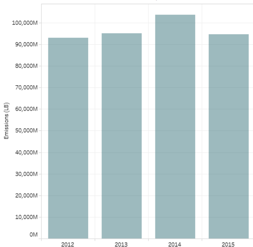
Annual emission totals, CO2-e
