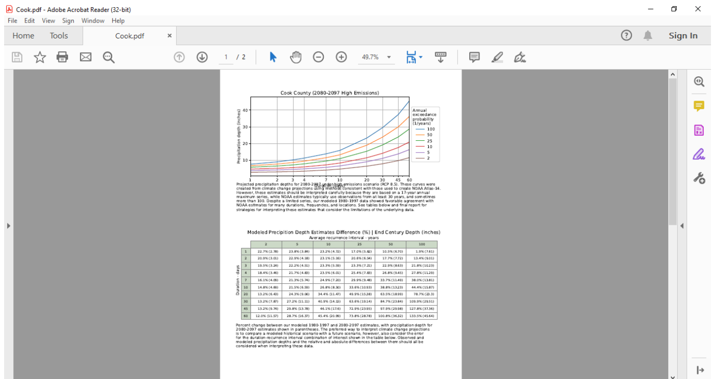
Image 6. Projected precipitation depths example from U of M Atlas-14 replication
